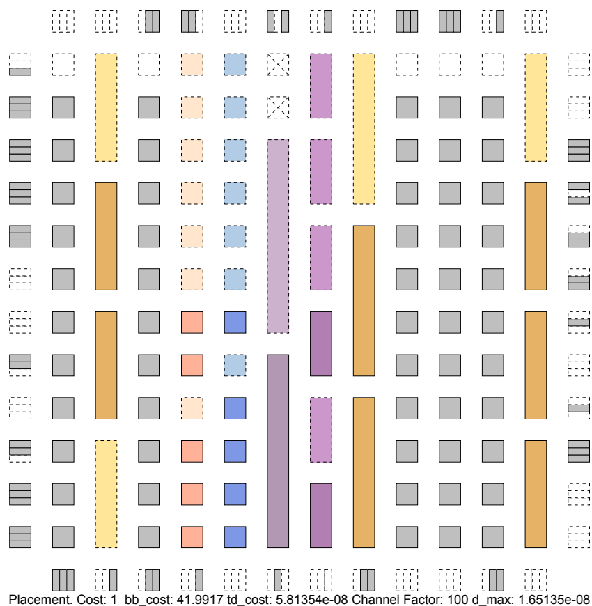
Fig. 7. A Heterogeneous FPGA in VPR 5.0
