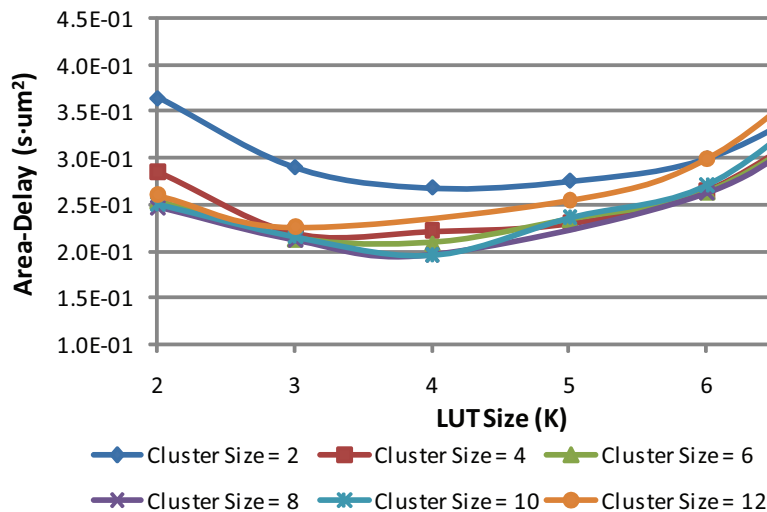
Fig. 10. Area-Delay vs Cluster and LUT Size
