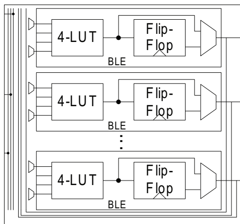
Fig. 2. Logic Cluster
