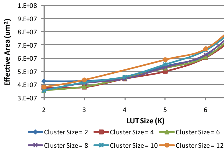
Fig. 8. Area vs. Cluster and LUT Size
