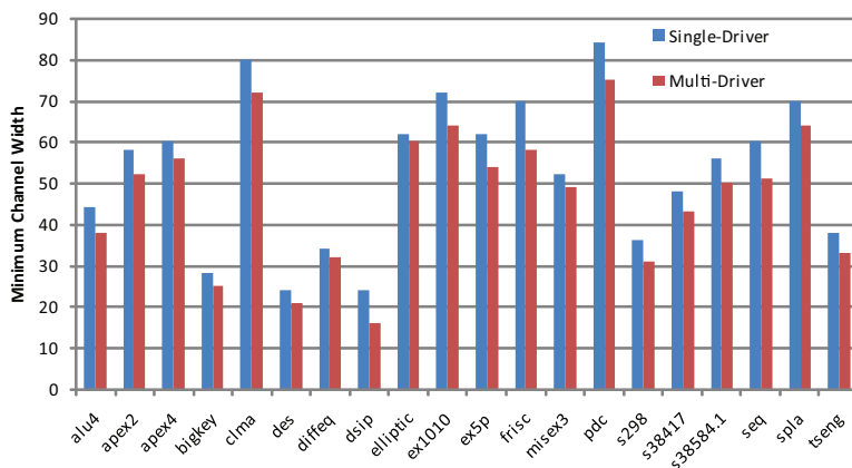
Fig. 6. Single- vs. Multiple-Driver Track Count
