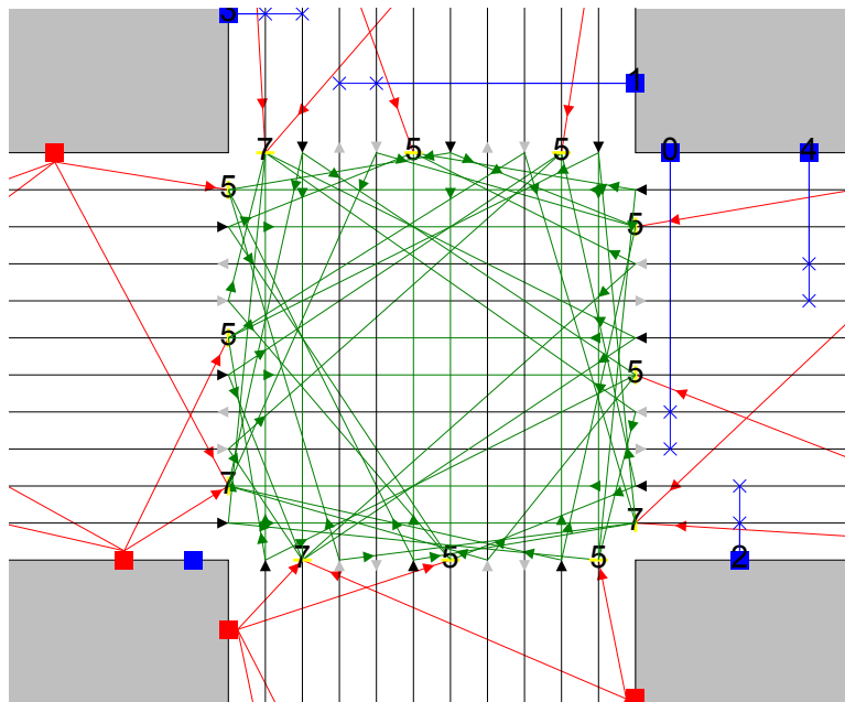
Fig. 5. Example Single-Driver Switch Block
