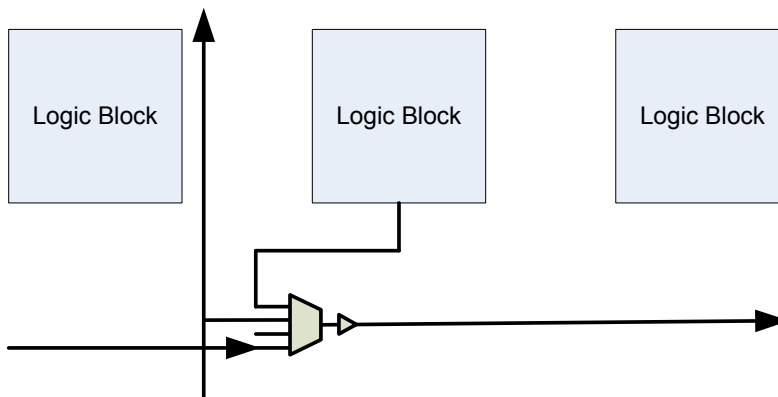
Fig. 4. Single Driver Routing
