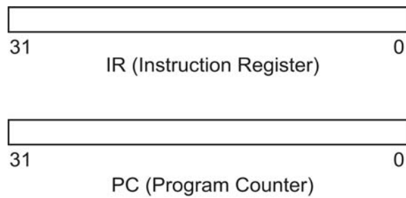
Figure 3: Internal Registers
